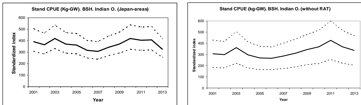
Figure 5. Standardized CPUEs obtained for sensitivity 1 (areas defined by Semba and Nishida 2008) and sensitivity 2 (without ratio) analyses for the blue shark during the 2001-2013 period, in the Indian Ocean.
