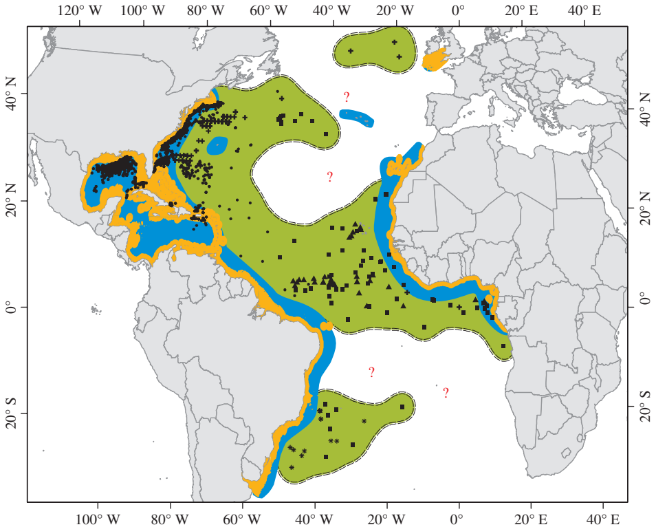
FIG. 1. Overlay of currently accepted distribution range of Galeocerdo cuvier (■, TIG range expansion IUCN, 2012) (■, Ebert et al. , 2013; ■, records obtained from observer and research programmes, and proposed extended distribution range in the Atlantic Ocean). ?, no positive records, but where occurrence is presumed given that there are no different conditions (★, Japan; ▲, Portugal; ■, Spain; ●, U.S.A.; ★, Uruguay).
